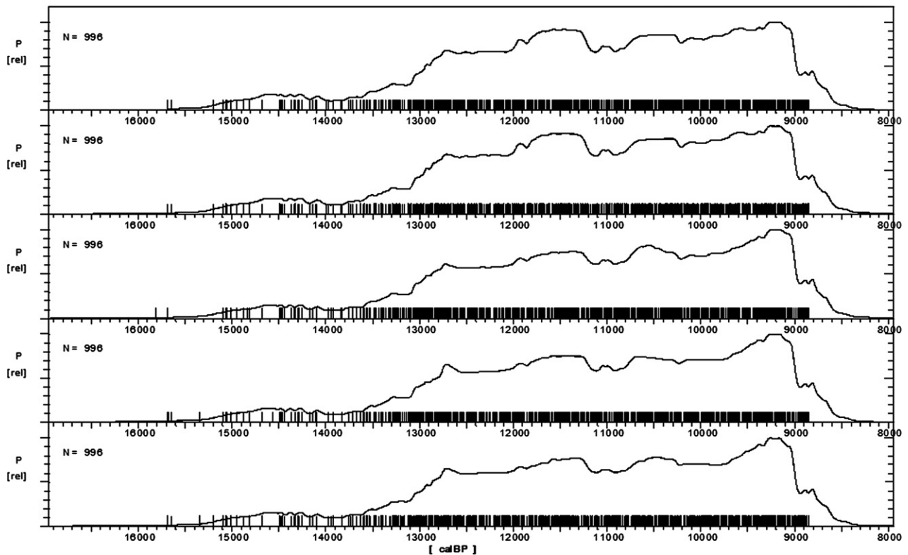
Fig. 1. Summed probability distributions derived from five random samples of 996 radiocarbon dates from Buchanan et al.'s (2008) original dataset.
