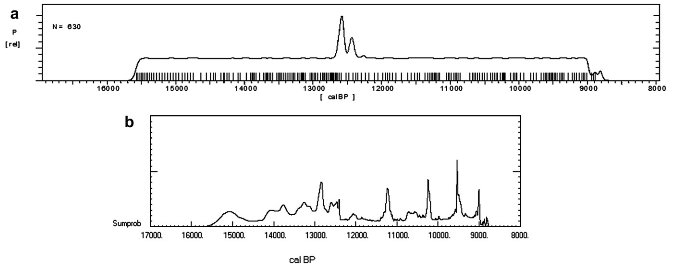
Fig. 3. Summed probability distributions generated from an artificial dataset of 630 uncalibrated radiocarbon dates designed to mimic a population spike. Top: Summed probability distribution calculated in CalPal using the IntCal04 calibration curve and the artificial dataset. Bottom: Summed probability distribution calculated in Calib 5.1 using the IntCal04 calibration curve.
