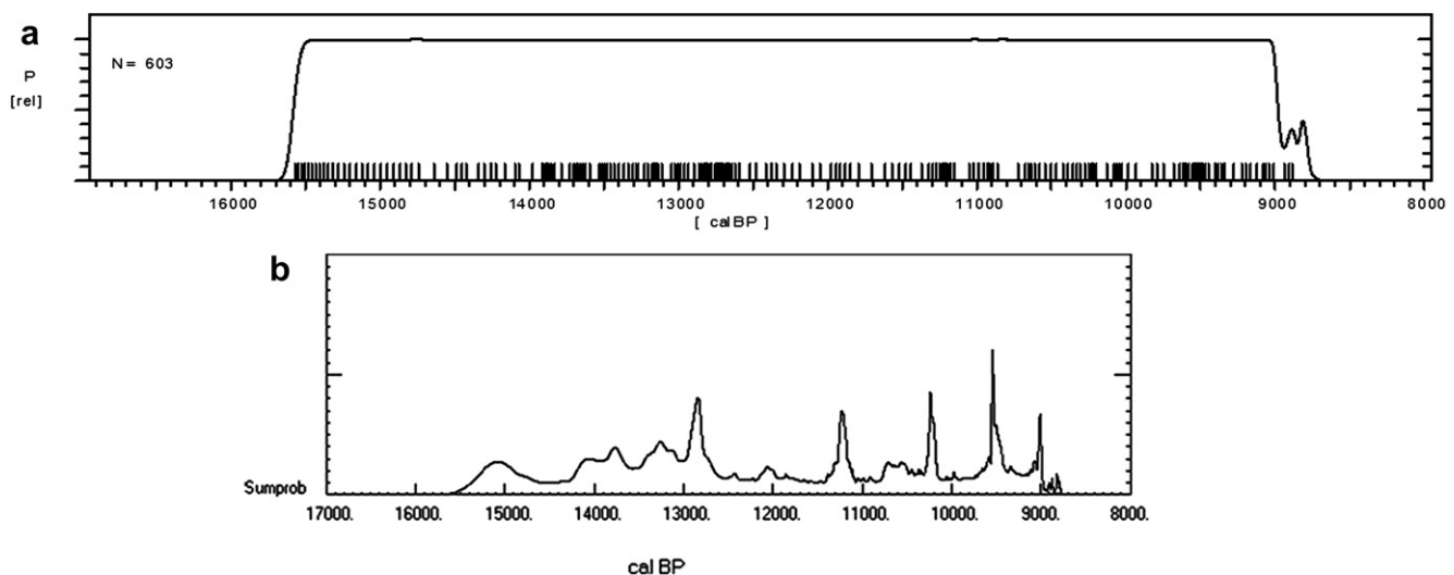
Fig. 2. Summed probability distributions generated from an artificial dataset of 603 uncalibrated radiocarbon dates designed to mimic an unchanging population. Top: Summed probability distribution calculated in CalPal using the IntCal04 calibration curve. Bottom: Summed probability distribution calculated in Calib 5.1 using the IntCal04 calibration curve.
