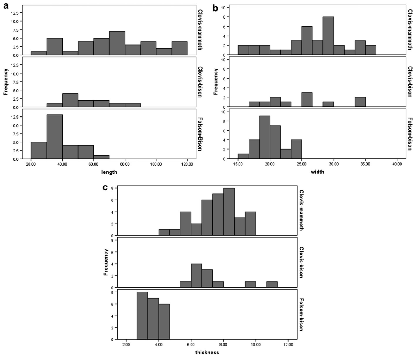
Fig. 8. Histograms for Clovis points associated with mammoth, Clovis points associated with bison, and Folsom points associated with bison for (a) length, (b) width, and (c) thickness measures.
